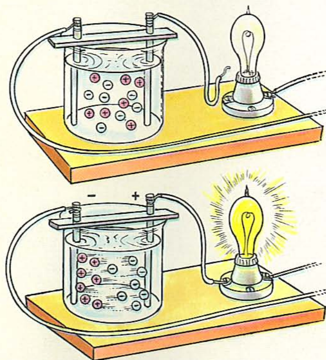
IN HIS EARLY EXPERIMENTS, SVANTE ARRHENIUS USED A SIMPLE SET-UP. YOU CAN EASILY REPEAT SOME OF HIS EXPERIMENTS IN YOUR OWN LAB, USING FLASHLIGHT BATTERIES.
